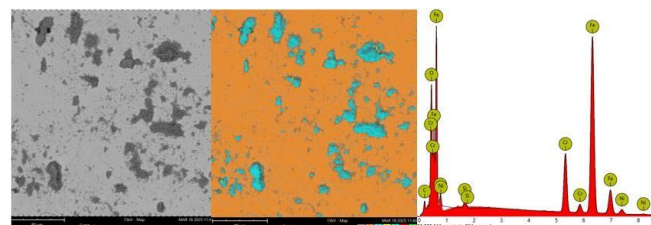
Figure 18. SEM analysis of worn anti-vibration bars-smooth anti-vibration bars in ambient air environment.
