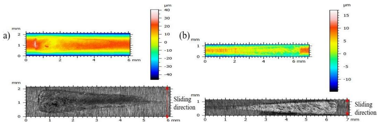
Figure 14. Impact wear morphology of 40 N: a) room-temperature air environment; b) room-temperature water environment.
