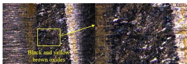
Figure 17. Abrasion marks morphology in a room-temperature water environment.
