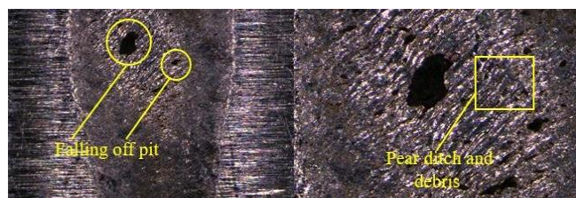
Figure 16. Abrasion marks morphology in a room-temperature air environment.
