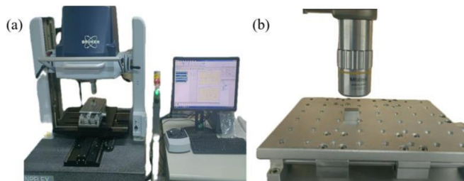
Figure 7. Nano-surface Interferometer: a) appearance of the equipment; b) observation platform.
