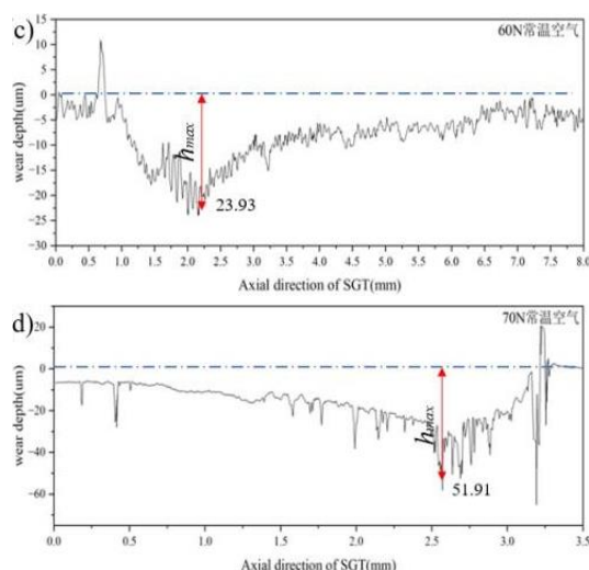
Figure 10. Quantitative analysis of thermal pipe wear under quasi-static vibration loads in ambient air: a)-d) 40-70 N.
