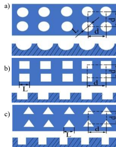
Figure 2. a) Circular dimple; b) square pit; c) triangular pit.
