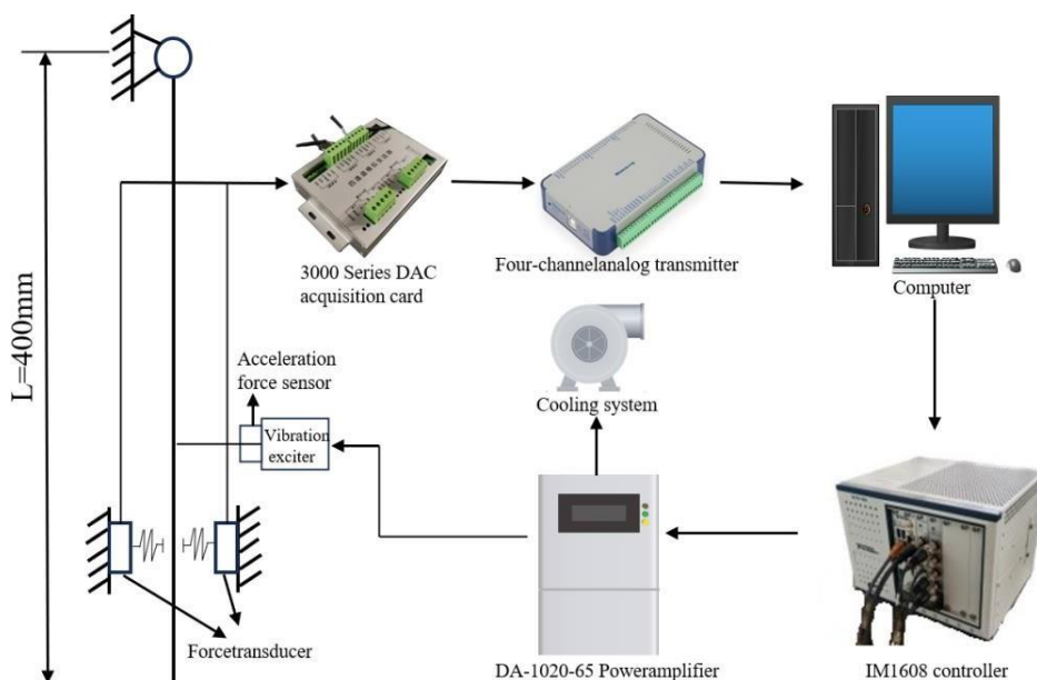
Figure 6. Flowchart of the wear test principle.
