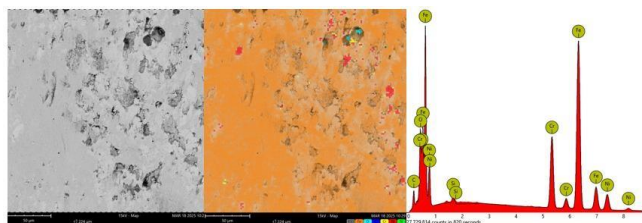
Figure 19. SEM analysis of worn anti-vibration bars-smooth anti-vibration bars in room-temperature water environment.
