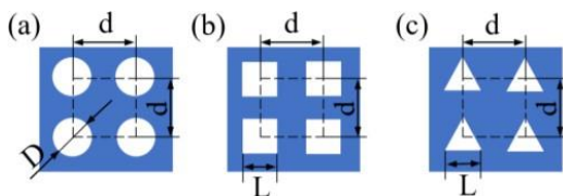
Figure 1. Schematic diagram for calculating micro-texture surface density: a) circular dimple micro-texture; b) square pit micro-texture; c) equilateral triangular pit micro-texture.
