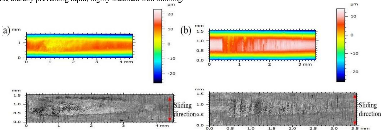
Figure 12. Impact wear morphology of 40 N: a) room-temperature air environment; b) room-temperature water environment.
