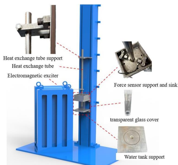
Figure 5. Physical picture of wear test device.
