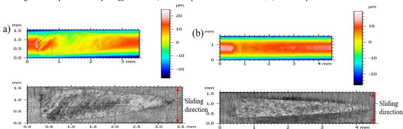
Figure 13. Impact wear morphology of 40 N: a) room-temperature air environment; b) room-temperature water environment.
