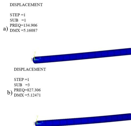
Figure 3. Simulation results of natural frequencies for a structure with one end fixed and the other end free: a) first-order natural frequency; b) second-order natural frequency.
