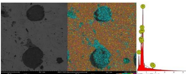
Figure 20. SEM analysis of worn anti-vibration bars-microtextured anti-vibration bars in room-temperature water environment.
