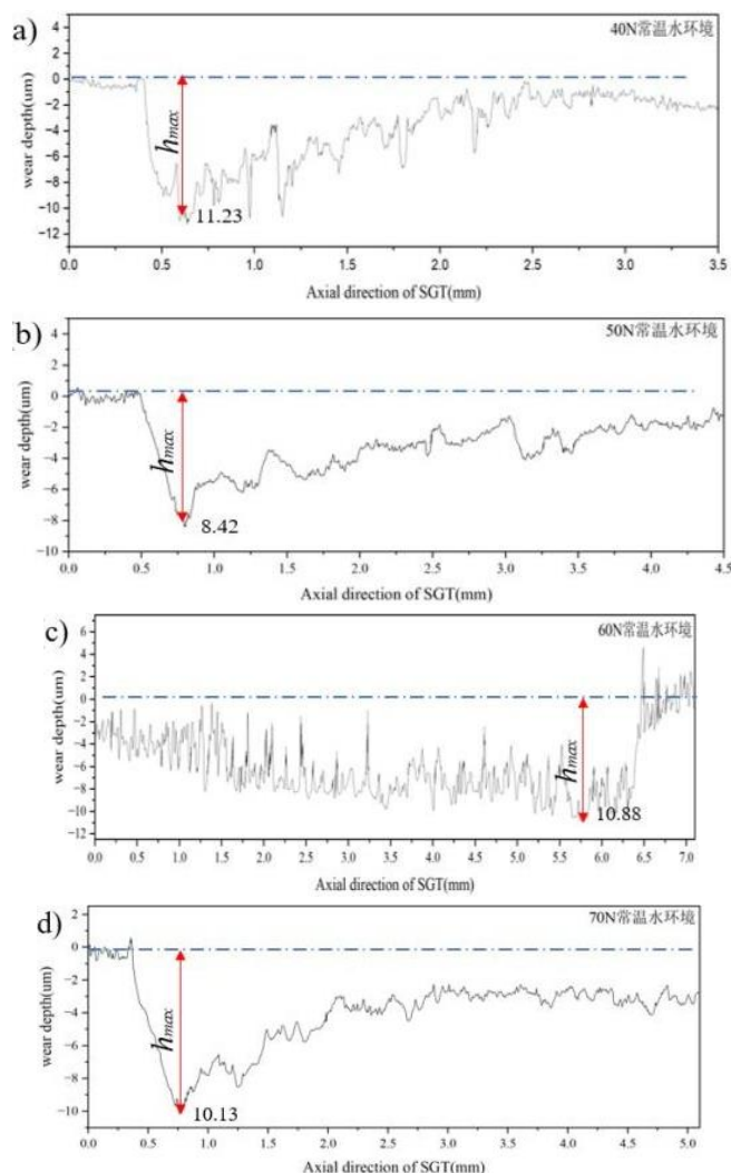
Figure 11. Quantitative analysis of heat exchanger tubing erosion under variable vibration loads in ambient water: a)-d) 40-70 N.
