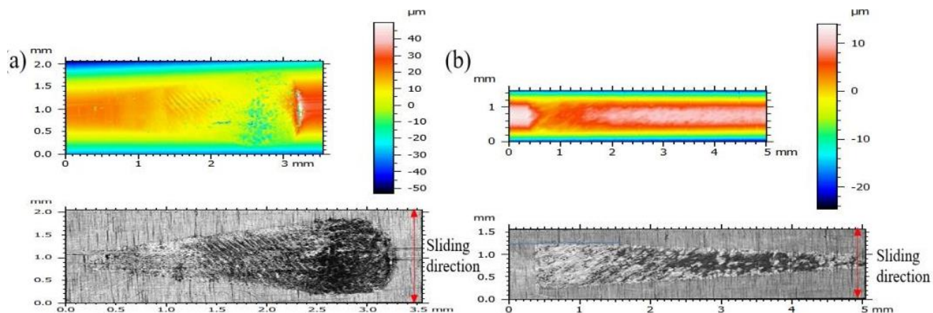
Figure 15. Impact wear morphology of 40 N: a) room-temperature air environment; b) room-temperature water environment.
