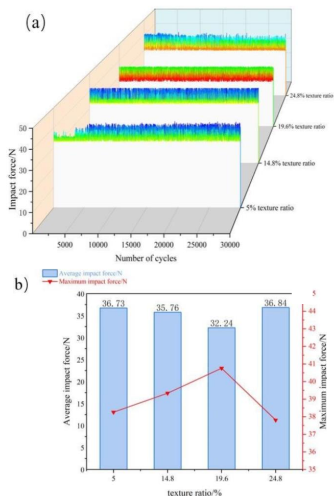
Figure 9. Impact force characteristics under different texture ratios: (a) cyclic impact force curves; (b) average and max. impact force
