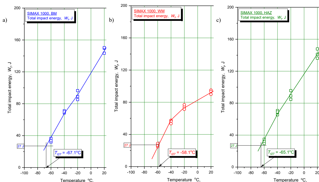
Figure 1. Dependence of total impact energy W_t on temperature: a) BM; b) WM; c) HAZ.
