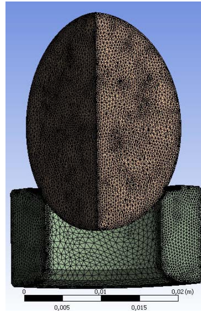
Figure 7. The meshing of 3D model of the valve (ball and seat). Slika 7. Mreža 3D modela ventila (kuglice i sedišta)
