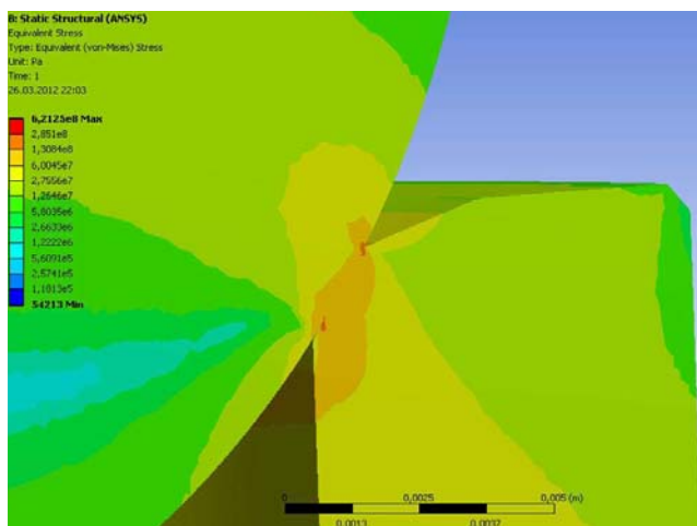
Figure 9. The state of equivalent stresses (von Mises criterion). Slika 9. Stanje ekvivalentnih napona (fon Mizesa)
