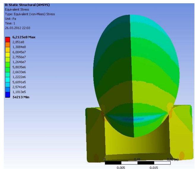
Figure 8. The state of equivalent stresses (von Mises criterion). Slika 8. Stanje ekvivalentnih napona (fon Mizesa)
