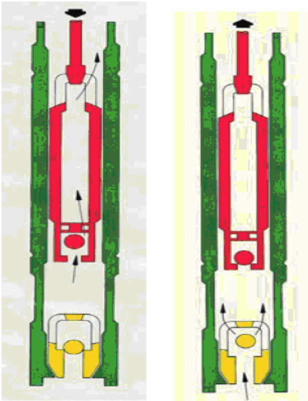
Figure 1. P-type and TB-type piston pumps. Slika 1. Pumpe tipa P i TB
